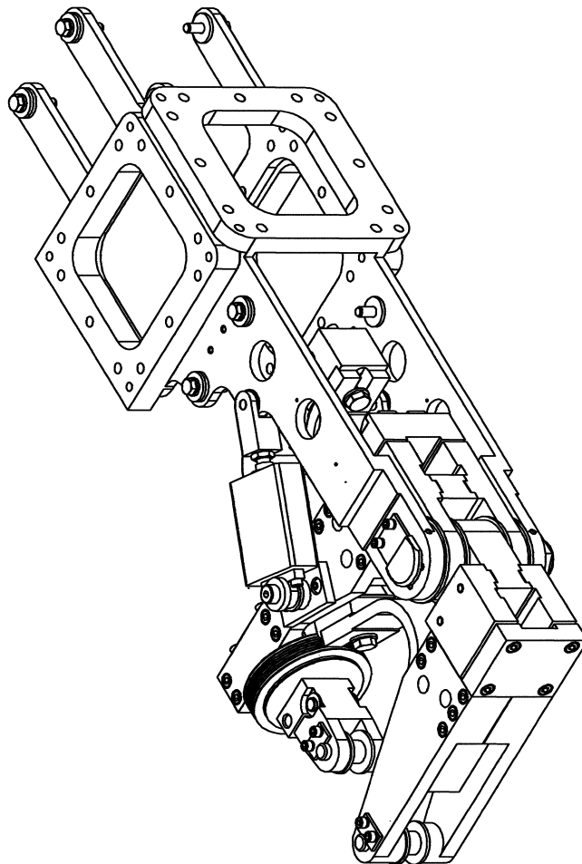
GROSSEL TOOL CO. SCISSOR TYPE / ROBOT STYLE BASE GUN ASSEMBLY "75076-11" & "75076-15"
